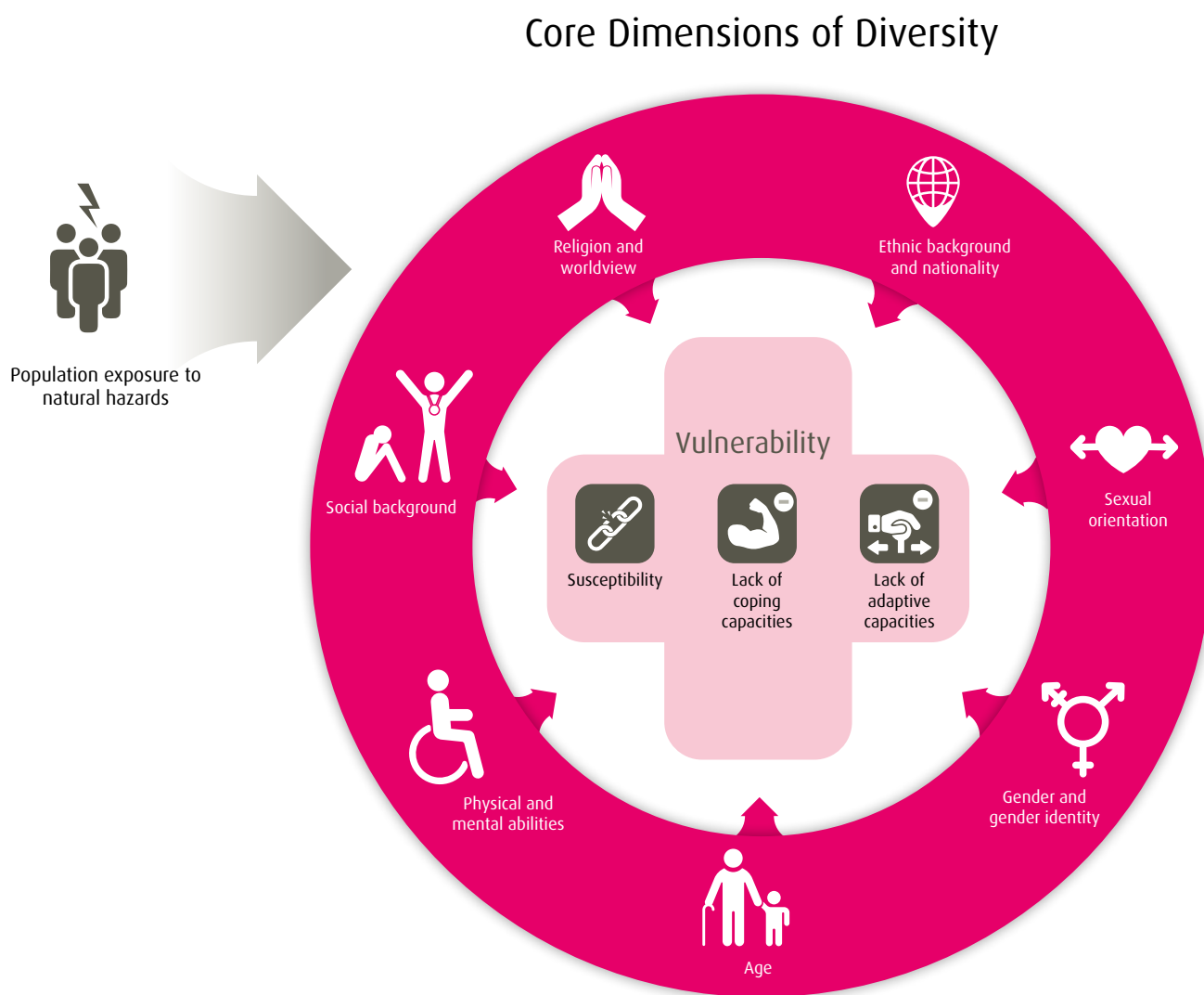
Figure 3: The seven core dimensions of diversity influence human vulnerability to extreme natural events.
